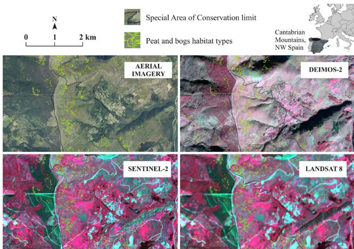
Figure 2. A detail of the study area (SAC Sierra del escudo, Cantabria Region) showing a 1:10000 vegetation map of peat and bogs classified as different habitat types (Annex I of Habitats Directive 92/43/EEC). Maps show the aerial photography and Deimos-2, Sentinel-2 and Landsat 8 imagery as a base map.
