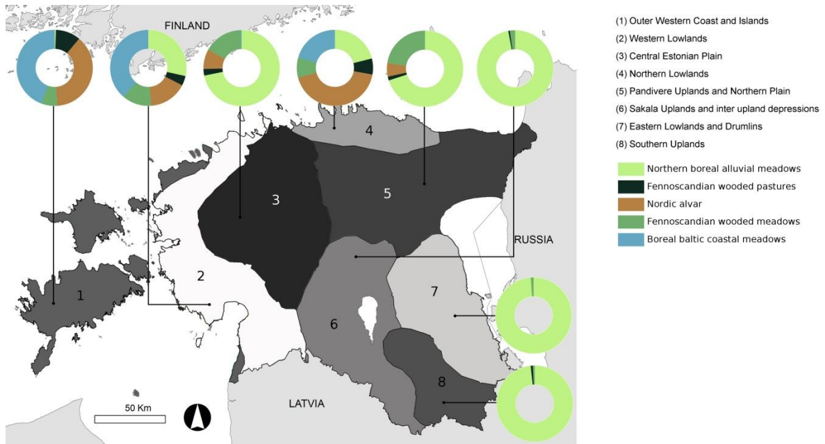
Fig 1. Share and distribution of semi-natural grassland habitats in Estonia. The calculations are based on the Environmental Stratification of Estonia (ESE) (Villoslada et al. 2016).
