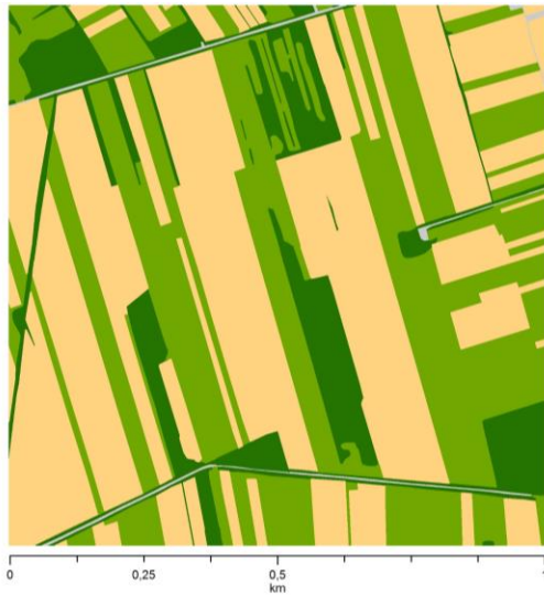
Landuse in Barje test area grey built-up orange fields green meadows dark green forests and overgrown areas
