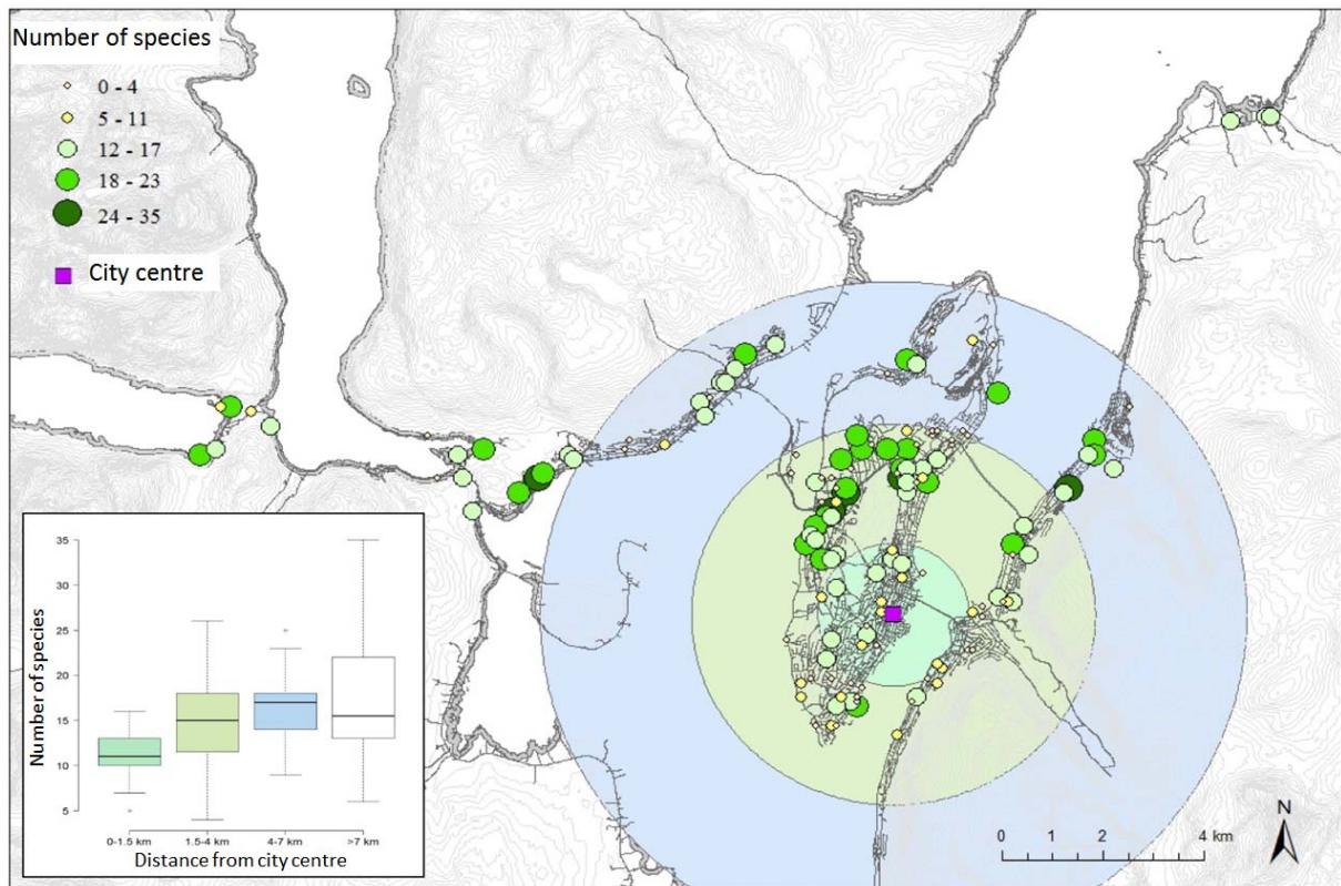
Figure 1: Number of species per 2 x 2m sample plot in unplanned green spaces of Tromsø City. The coloured rings indicate distance from the city centre (dark green at the centre, light green from 1.5 km to 4 km, blue from 4 – 7 km and white beyond 7 km).
