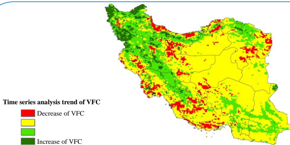
Distribution changes of time series analysis trend of VFC
