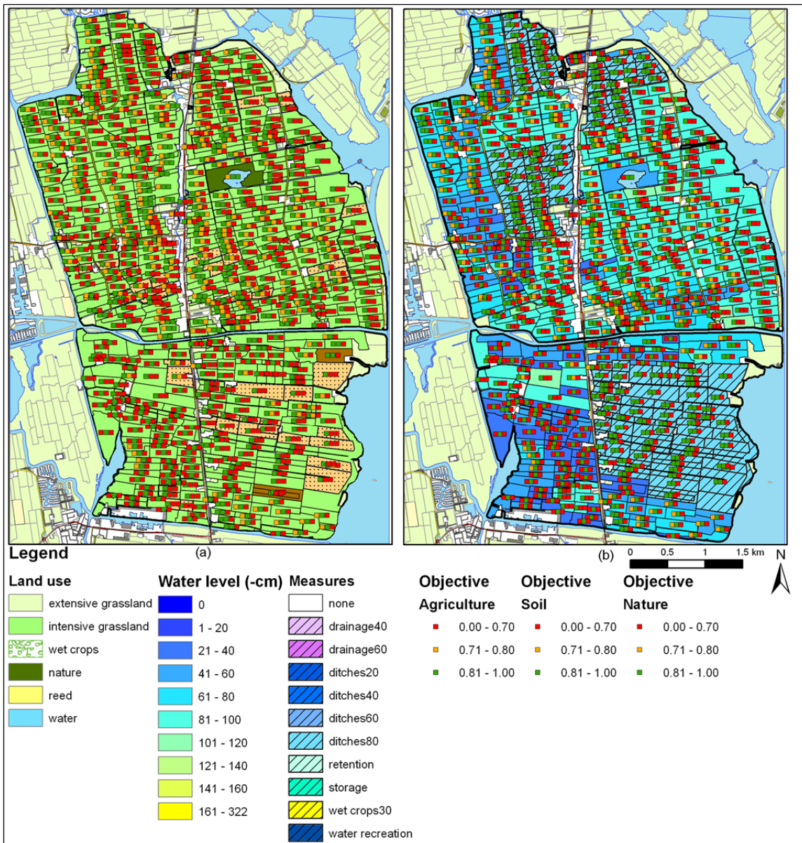
Figure 2 Use of the design tool for the region 'Hommerts': combined with land use (a) and water levels (b)
